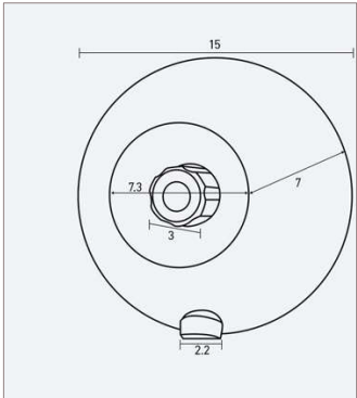
UC40 quarter turn
