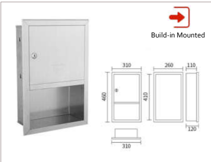
UL46 Paper Towel Dispenser 460*312*120mm
