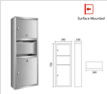
UL75-A 750*300*140mm surface mounted
