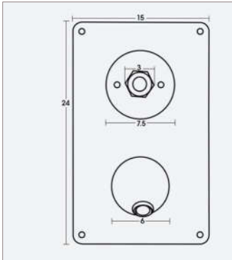
UC42 shower set
