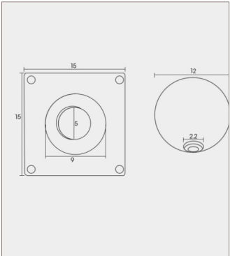
UC430 shower set
