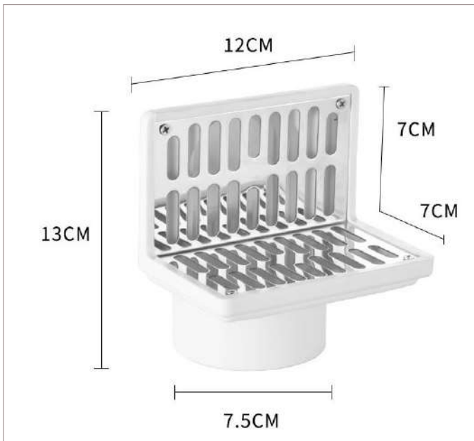
D420 corner L shape drain Pvc house 304 stainless steel linear
