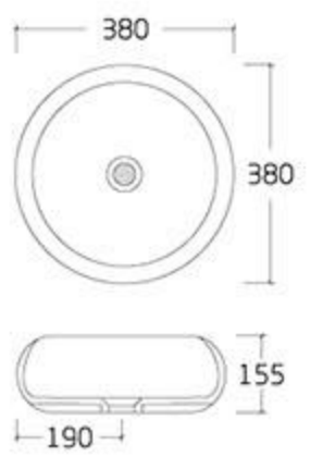
type: Art basin 0715A-B3 380*380*155mm
