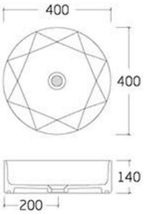
type: Art basin 6182-3 400*400*140mm
