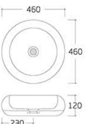
type: Art basin 0547 460*460*120mm 0544 510*510*110mm
