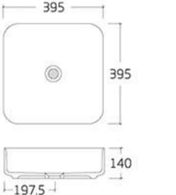
type: Art basin 78110-M5 395*395*140mm
