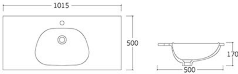
type: Cabinet basin N-100 1015*500*170mm NEW
