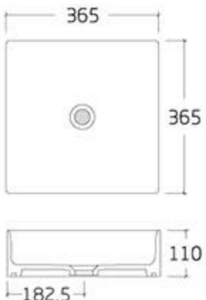
type: Art basin 78110C-AM 365*365*110mm
