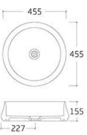
type: Art basin 6188-3 455*455*155mm
