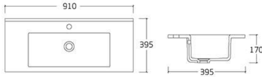
type: Cabinet basin 9039 910*395*170mm
