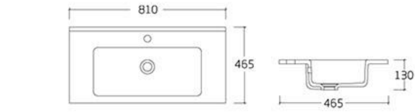
type: Cabinet basin E-80 810*465*130mm
