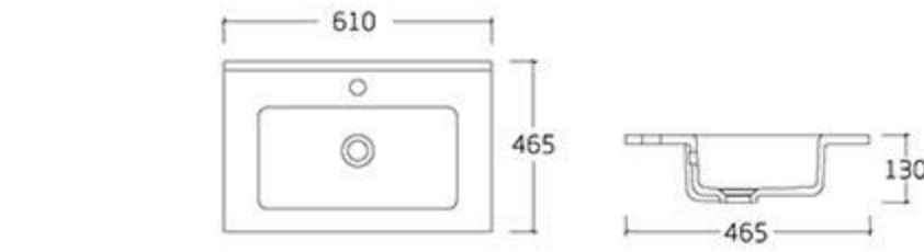
type: Cabinet basin E-60 610*465*130mm
