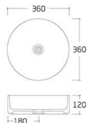
type: Art basin 6182-C5 360*360*120mm
