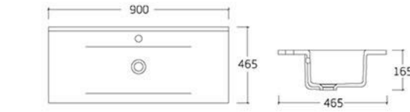
type: Cabinet basin B90 900*465*165mm
