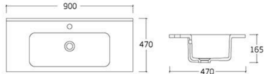
type: Cabinet basin 90B 900*470*165mm
