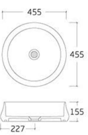
type: Art basin 6188-4 455*455*155mm
