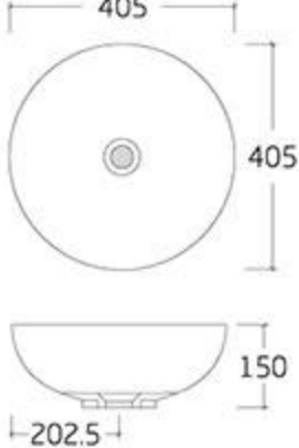
type: Art basin 78129-M4 405*405*150mm
