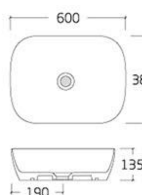
type: Art basin LB152-BW 600*380*135mm 500*380*135mm
