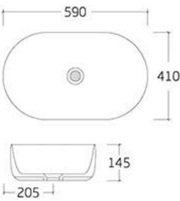
type: Art basin 0836-M2 590*410*145mm
