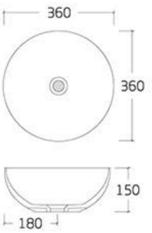
type: Art basin LB135-BM 360*360*150mm
