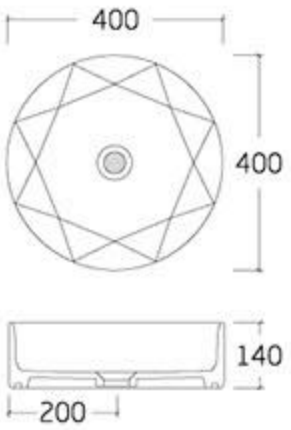
type: Art basin 6182-2 400*400*140mm
