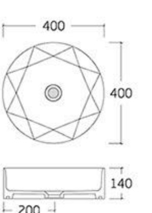
type: Art basin 6182-E5 400*400*140mm
