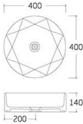
type: Art basin 6182-C1 400*400*140mm
