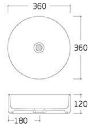
type: Art basin 78120-MP 360*360*120mm
