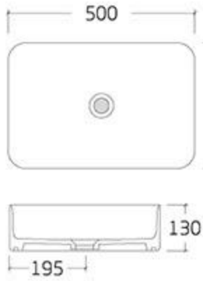
type: Art basin 78109-DGM 500*390*130mm
